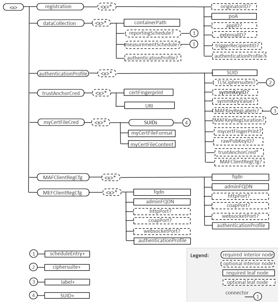
Figure 1: Figure 5.6.2-1: Structure of OMA-DM compatible M2M FieldDevice-Config MO (MFDCMO)
