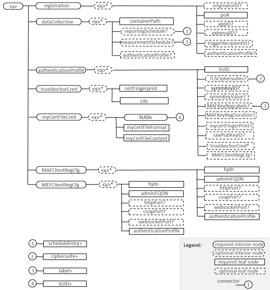
Figure 1: Figure 5.6.2-1: Structure of OMA-DM compatible M2M FieldDevice-Config MO (MFDCMO)
